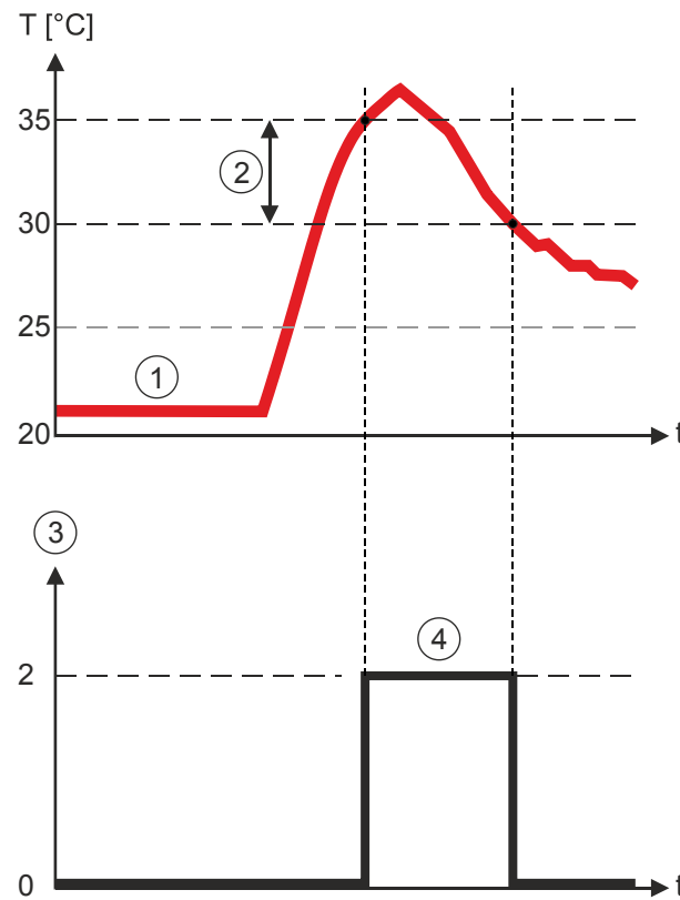
Figure 10: Ambient supervision output signal when the operating temperature threshold value of 35 °C is exceeded and a hysteresis range of 5 °C is selected. The diagram below shows the progression of the output signal.
