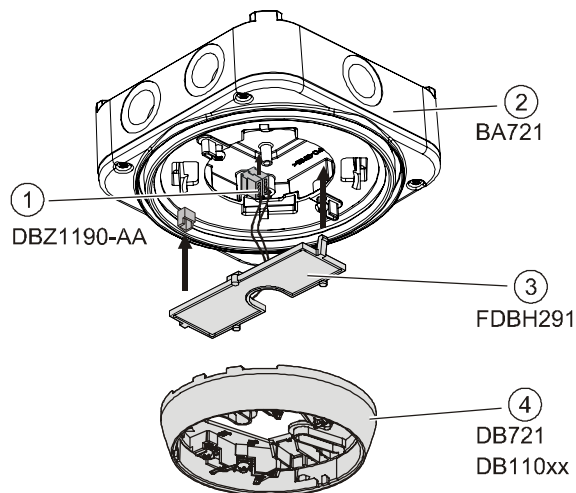
Figure 21: Mounting of the detector heating unit FDBH291
