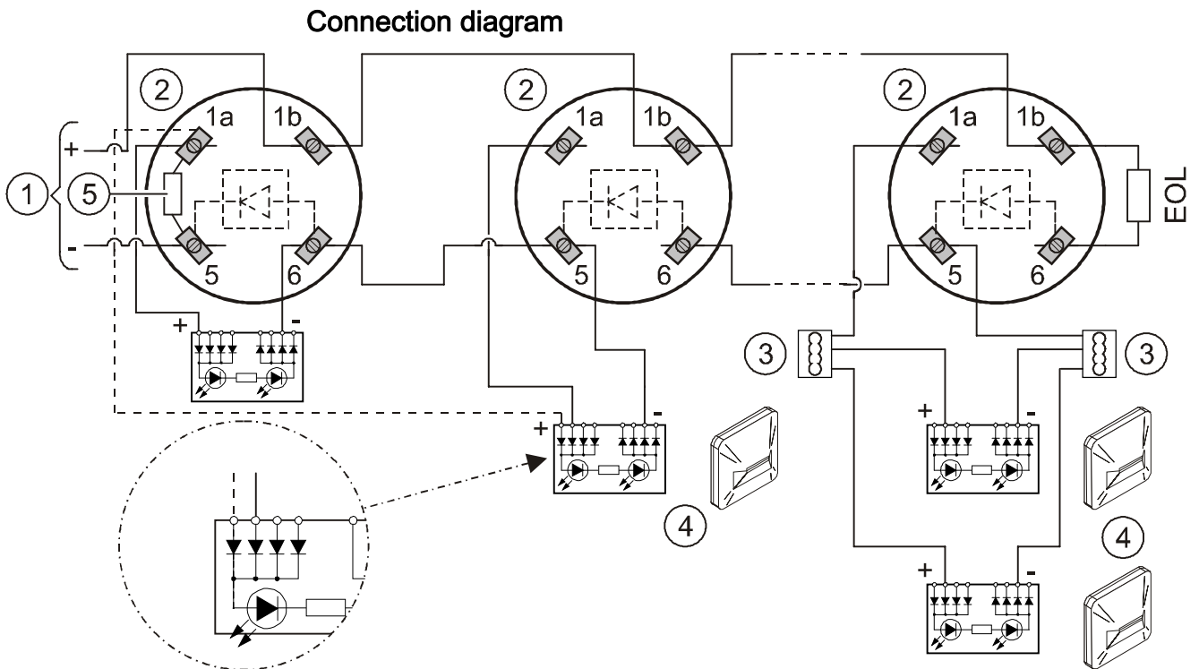
Figure 20: Connection diagram for collective detector lines
