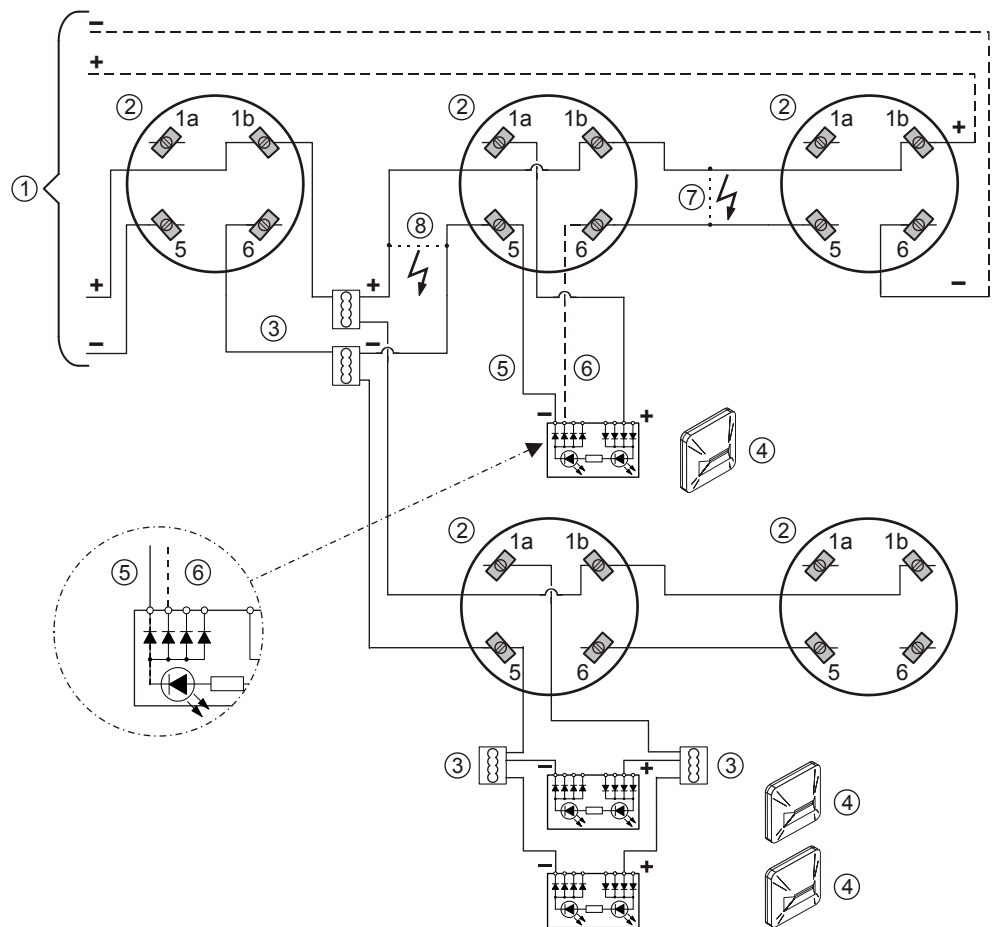
Figure 19: Connection diagram for addressed detector lines
